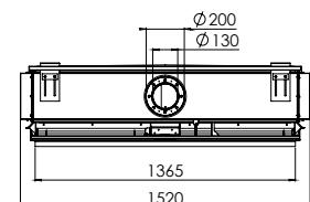
Metro 130XT | Tunnel (P. 44, 48)
