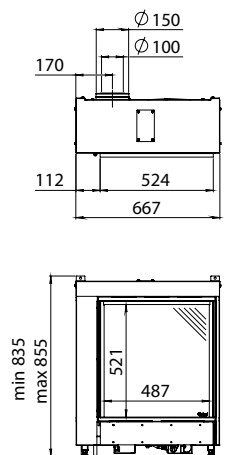
Global 55XT Cavity BF (P. 78)
