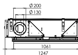
Metro 100XT | Tunnel (P. 43, 47)
