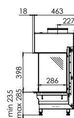
Metro 100XT | Tunnel (P. 43, 47)
