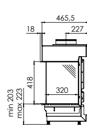
Metro 80XT | Tunnel (P. 42, 46)
